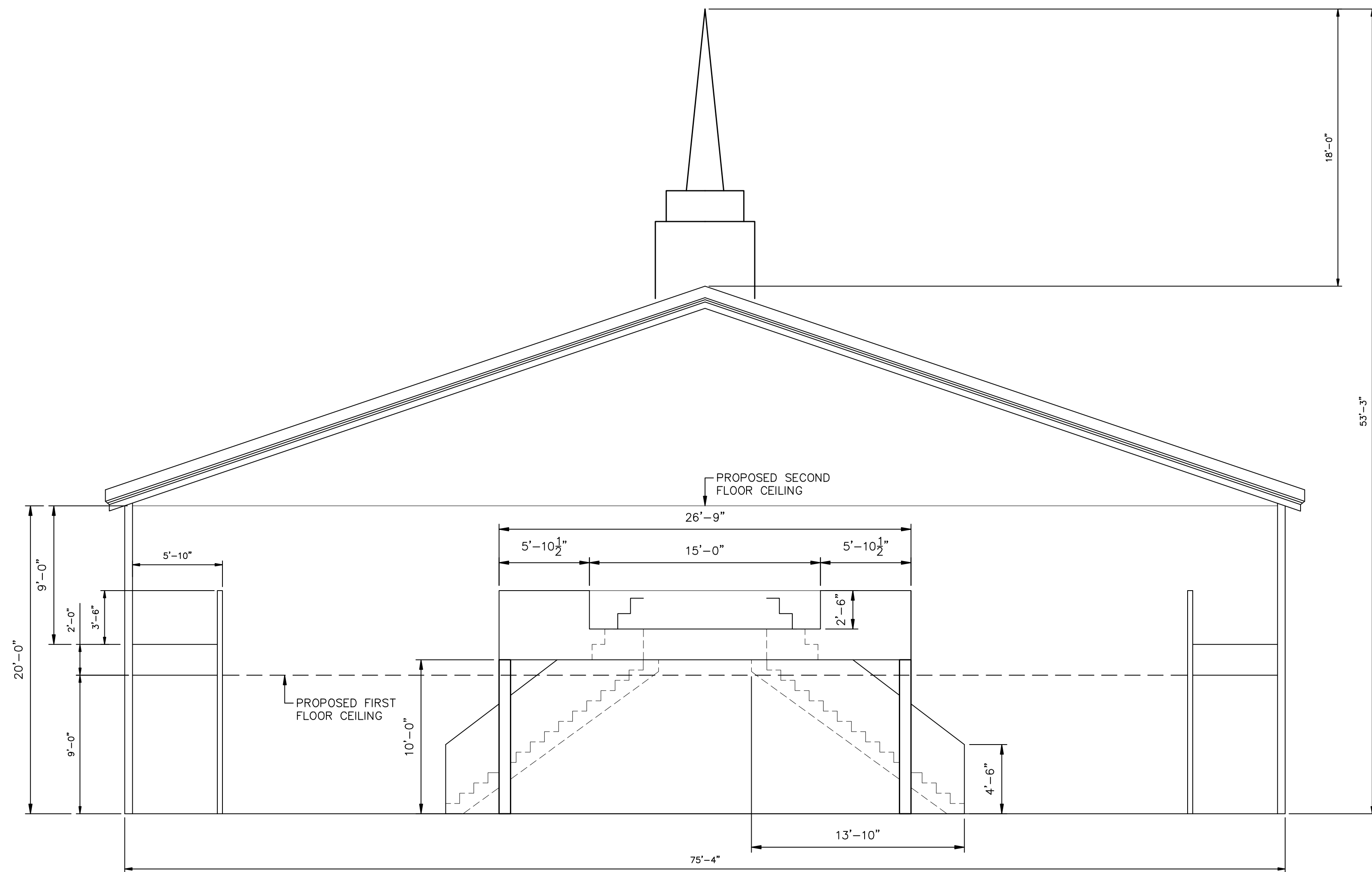
1 BUILDING SECTION SCALE: 3/16" = 1'-0"
