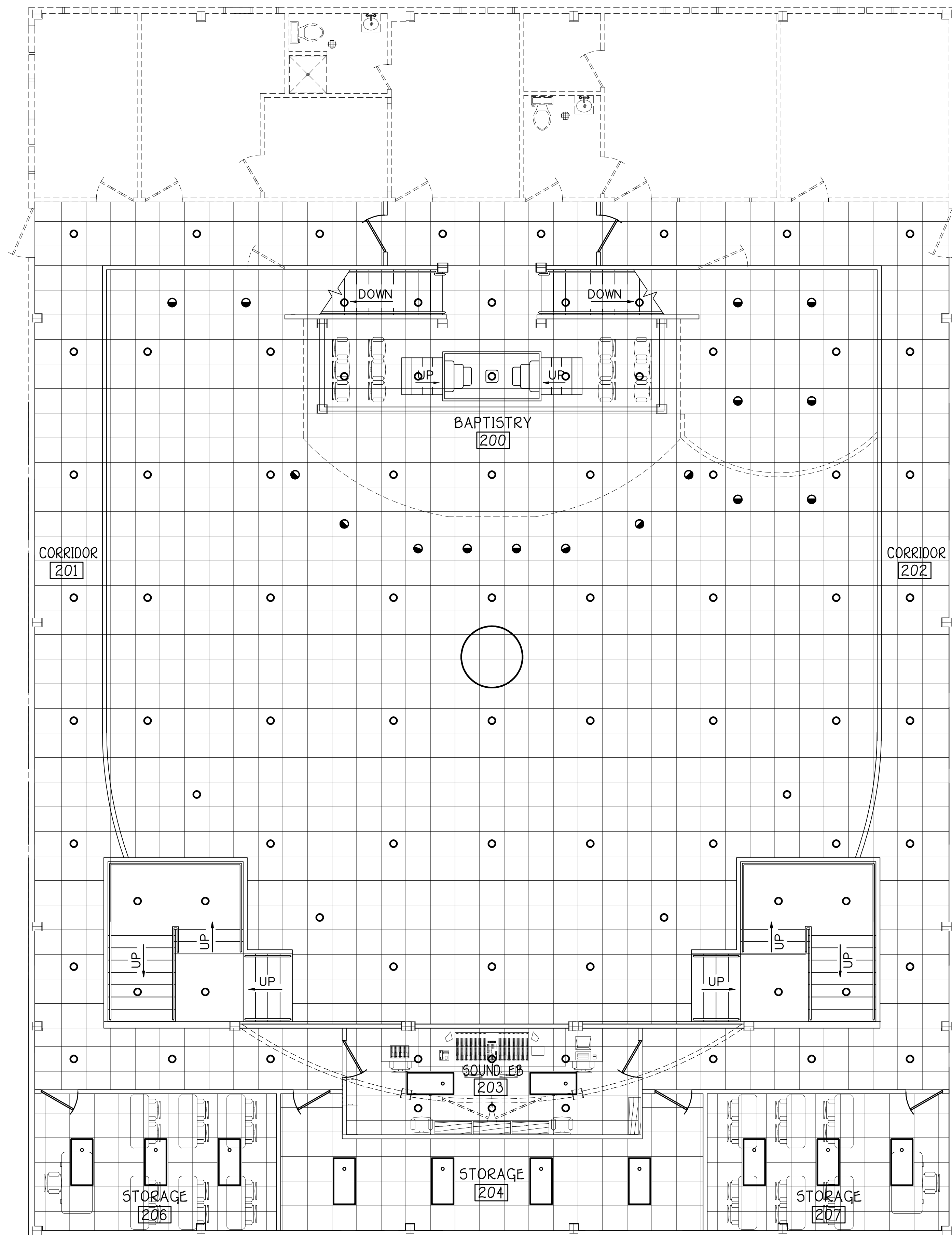
1 LIGHTING SECOND FLOOR PLAN SCALE: 3/16" = 1'-0"
